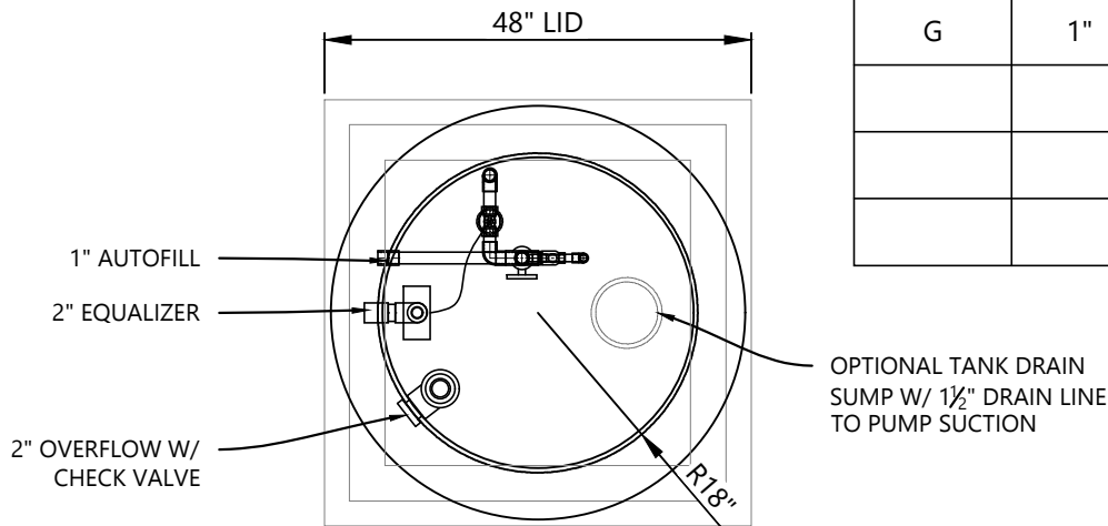
PLAN VIEW
