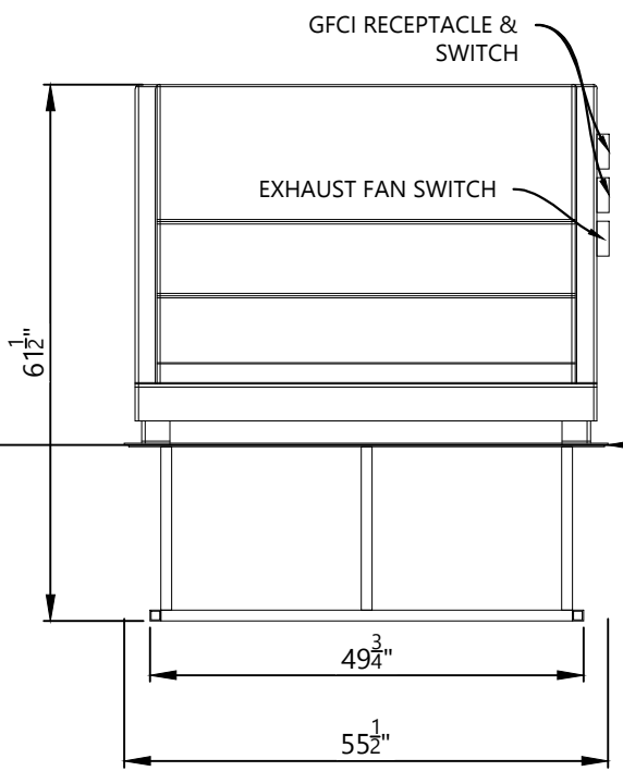
EQUIPMENT PACK FRONT ELEVATION
