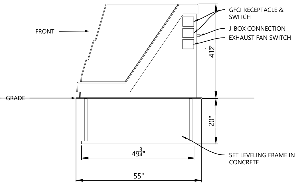
EQUIPMENT PACK SIDE ELEVATION
