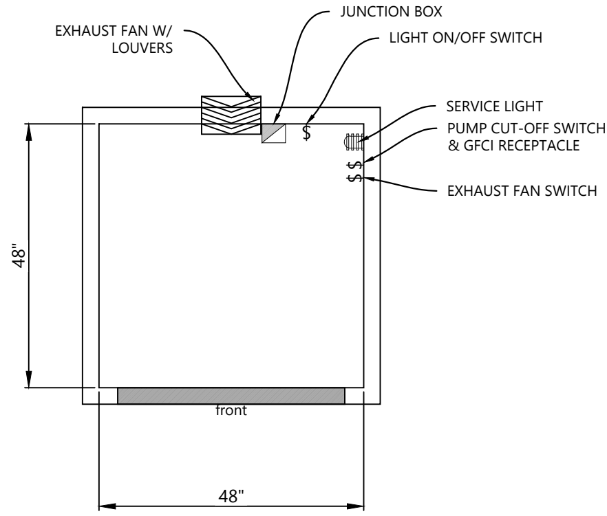
EQUIPMENT PLAN
